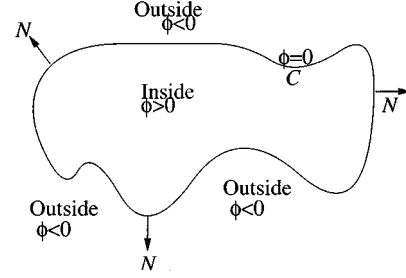
Fig. 2. Curve C = \{(x, y) : \phi(x, y) = 0\} propagating in normal direction.
