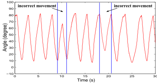
Figure 5. A typical measurement signal (angle) from inertial sensor for the chair-stand test
