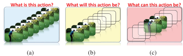
Figure 1. (a) Traditional action recognition/retrieval with full observations; (b) action prediction with partial observations at the beginning; (c) partial action recognition/retrieval with observations at any time (if partial observations are very limited and of unknown observation ratios, this turns into our problem).
