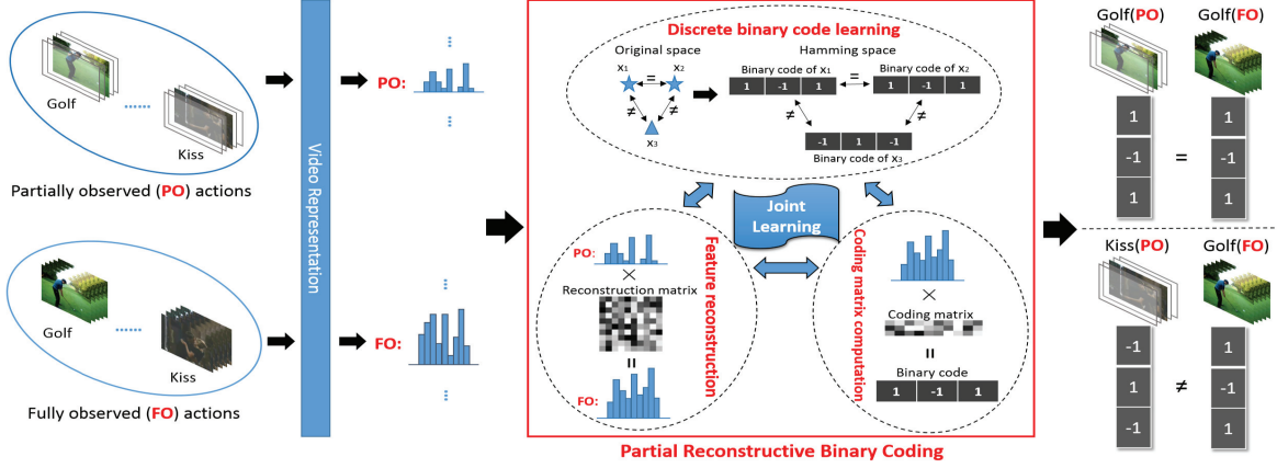
Figure 2. The overall framework of PRBC. We collaboratively learn a joint framework for feature reconstruction and binary coding. The learned binary codes are similarity-preserving and discriminative for action recognition/retrieval from partially observed actions.
