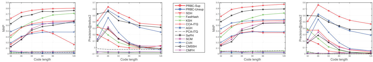
Figure 5. Retrieval results on UCF101 using 16-frame (left two figures) and 32-frame (right two figures) partial actions as queries.
