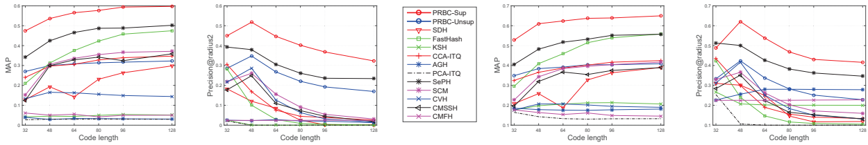
Figure 4. Retrieval results on HMDB51 using 16-frame (left two figures) and 32-frame (right two figures) partial actions as queries.
