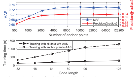
Figure 3. Evaluation of AAS on UCF101. The Mean Average Precision (MAP) and precision within Hamming radius 2 are reported using 48-bit codes. The total number of training points is 123,200.
