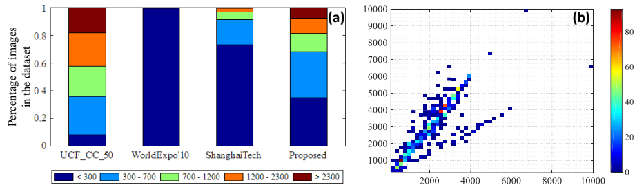
Fig. 2: (a) This graph shows the relative distribution of image counts among the four datasets. The proposed UCF-QNRF dataset has a fair number of images from all five count ranges. (b) This graph shows a 2D histogram of image resolution for all the images in the new dataset. The x-axis shows the number of rows, while y-axis is the number of columns. Each bin ( 500 \times 500 pixels) is color-coded with the number of images that have the corresponding resolution.
