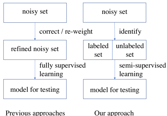
Figure 1. Comparison between our framework and the one of existing methods for learning from noisy labels. Instead of trying to correct or reweigh all the labels of the noisy data, we ignore the ambiguous ones and train a deep neural network in a semi-supervised fashion.
