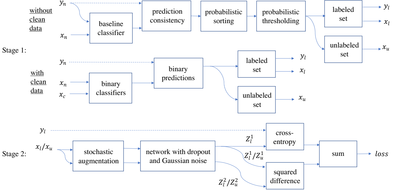
Figure 2. Overview of the two stages in our approach. In Stage 1, we mine some examples from the noisy training set such that their labels are more likely correct than the others'. After that, we employ a semi-supervised learning method in Stage 2 to train a deep neural network. We use the subscripts n and c to represent the noisy and clean data, respectively. The subscripts l and u respectively stand for the labeled and unlabeled data points that are identified by Stage 1 and then input to Stage 2.
